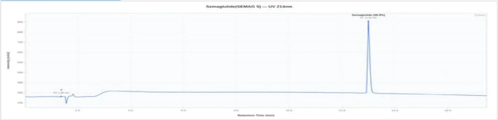
Semaglutide SEMAG 5 - LOT-2026-332: UV Chromatogram
