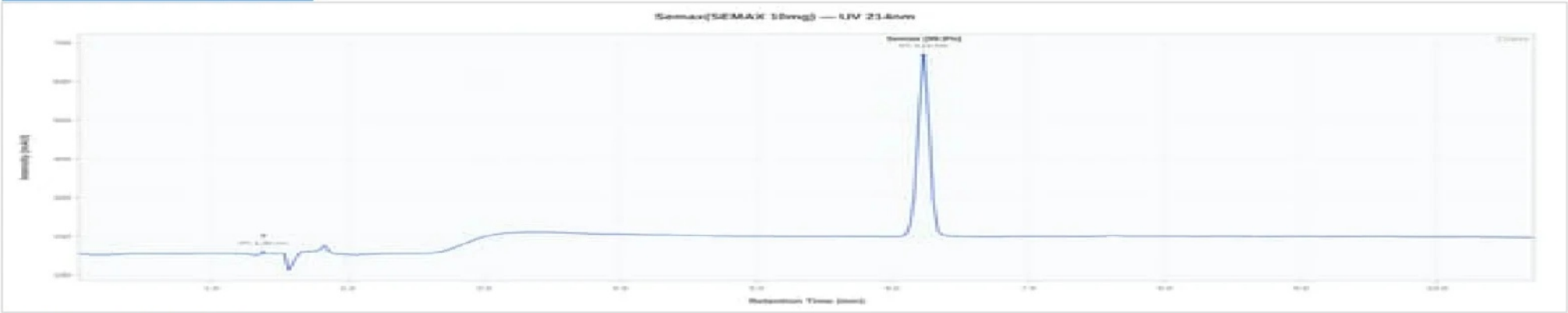
SEMAX 10mg - LOT-2026-332: UV Chromatogram
